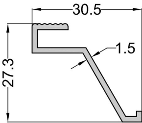
NO : 94-529 0.240 Kg.m.
