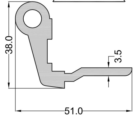
NO : 94-603 1.170 Kg.m.
